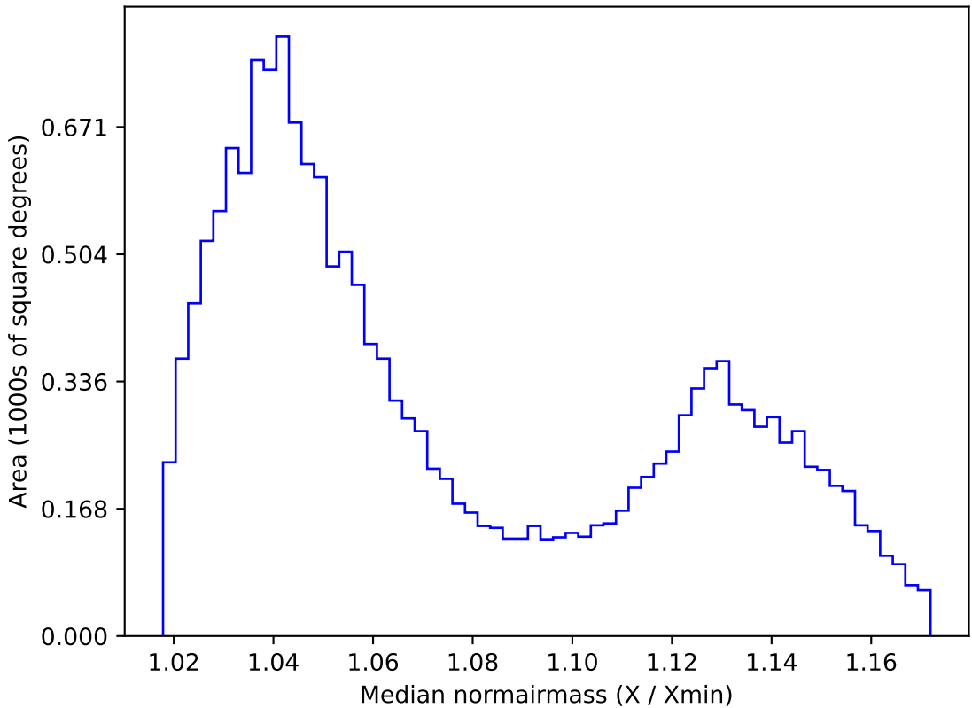
extra_ss_neo4_v3.4_10yrs WFD i band: Median normairmass
