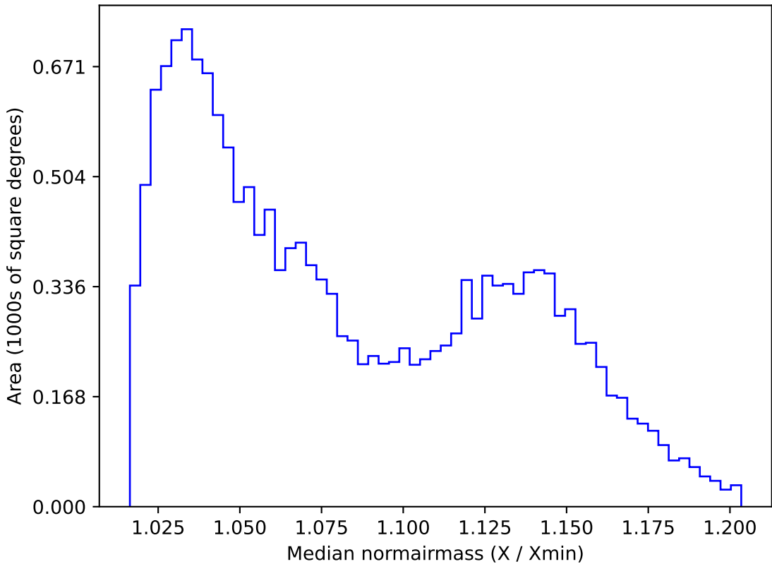
extra_ss_neo4_v3.4_10yrs WFD g band: Median normairmass
