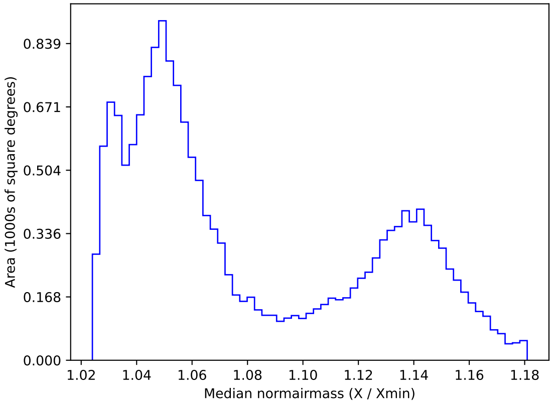
extra_ss_neo4_v3.4_10yrs WFD all bands: Median normairmass
