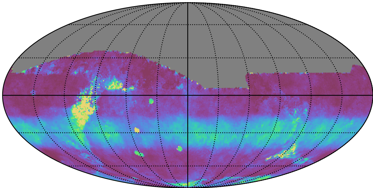
extra_ss_neo4_v3.4_10yrs All sky z band: Median normairmass
