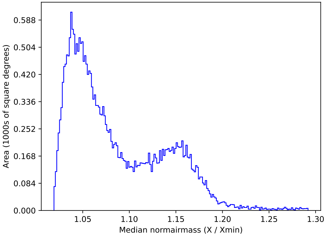
extra_ss_neo4_v3.4_10yrs All sky z band: Median normairmass
