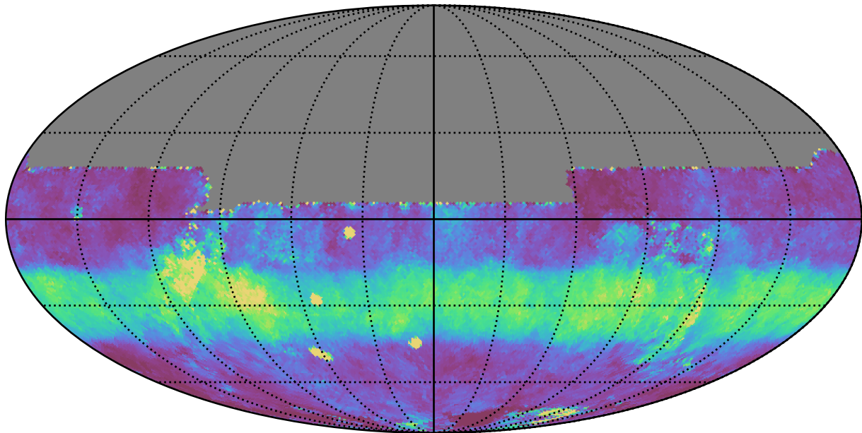
extra_ss_neo4_v3.4_10yrs All sky y band: Median normairmass
