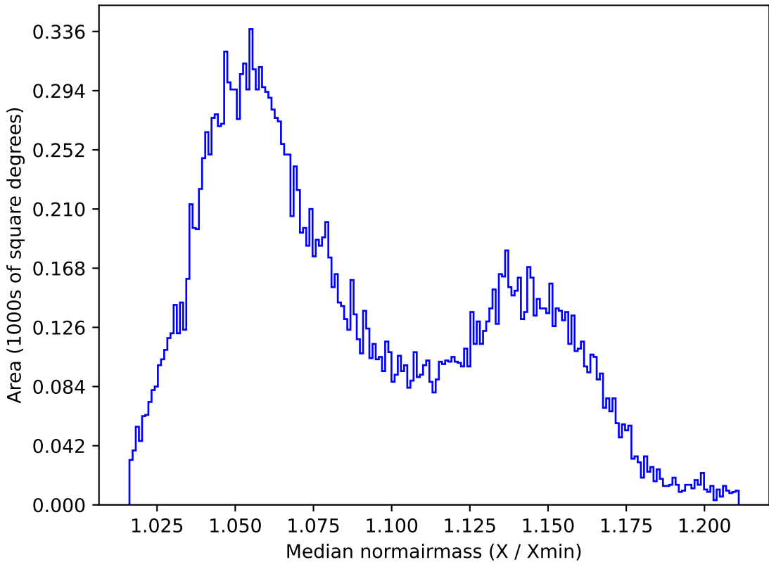
extra_ss_neo4_v3.4_10yrs All sky y band: Median normairmass
