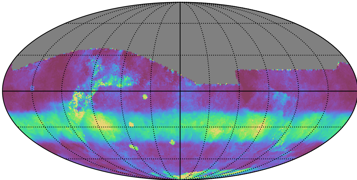
extra_ss_neo4_v3.4_10yrs All sky r band: Median normairmass
