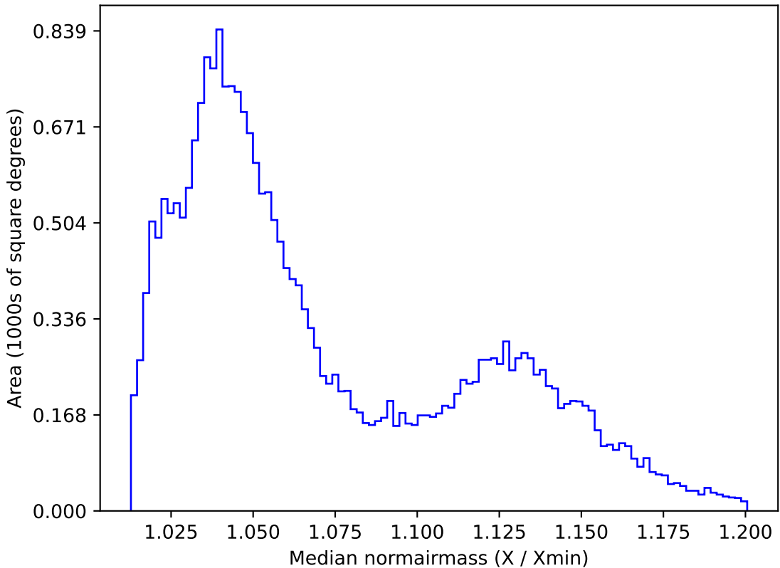
extra_ss_neo4_v3.4_10yrs All sky r band: Median normairmass
