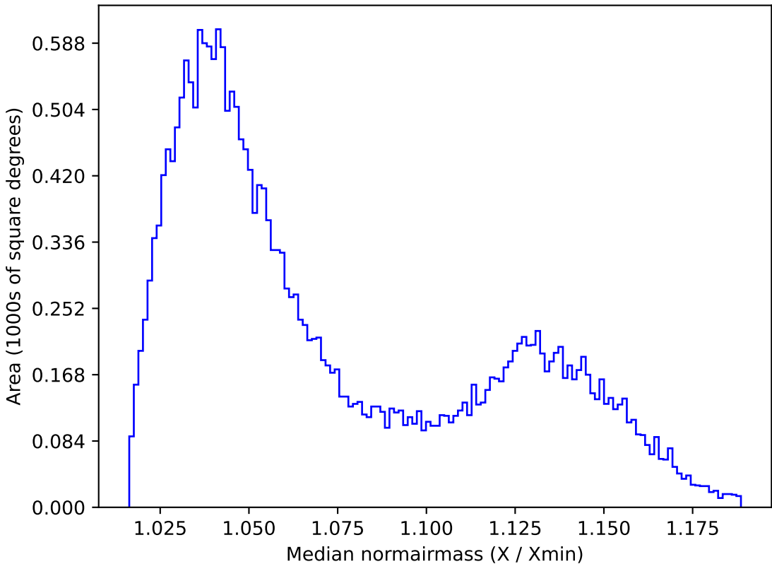
extra_ss_neo4_v3.4_10yrs All sky i band: Median normairmass
