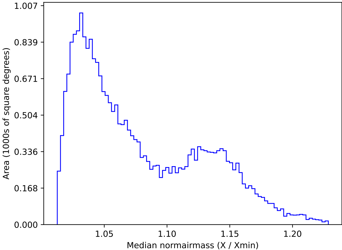
extra_ss_neo4_v3.4_10yrs All sky g band: Median normairmass
