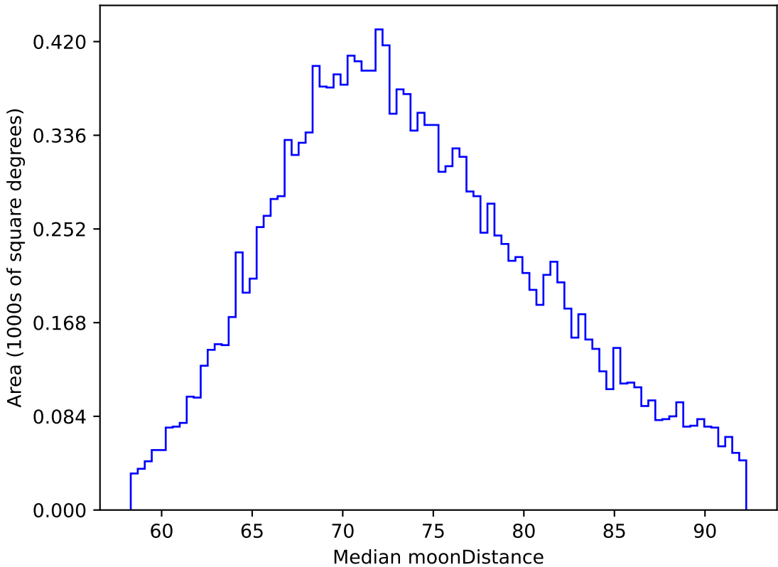
extra_ss_neo4_v3.4_10yrs WFD z band: Median moonDistance
