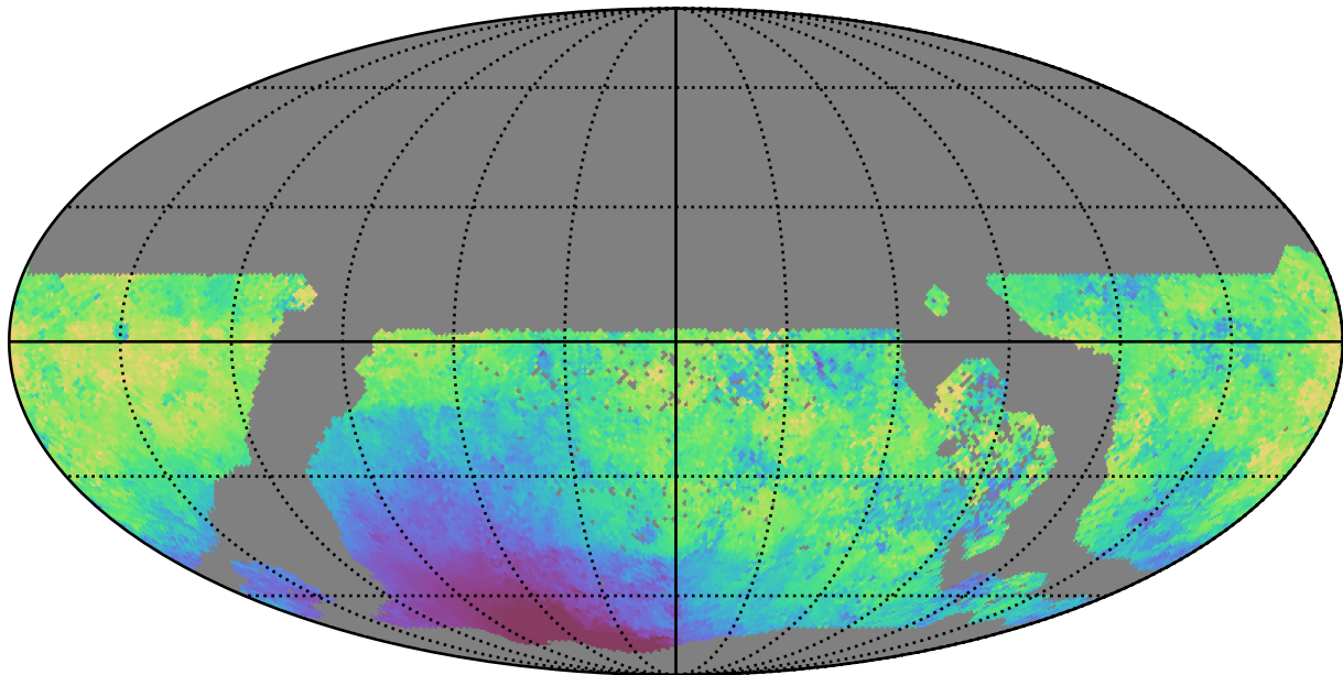
extra_ss_neo4_v3.4_10yrs WFD u band: Median moonDistance
