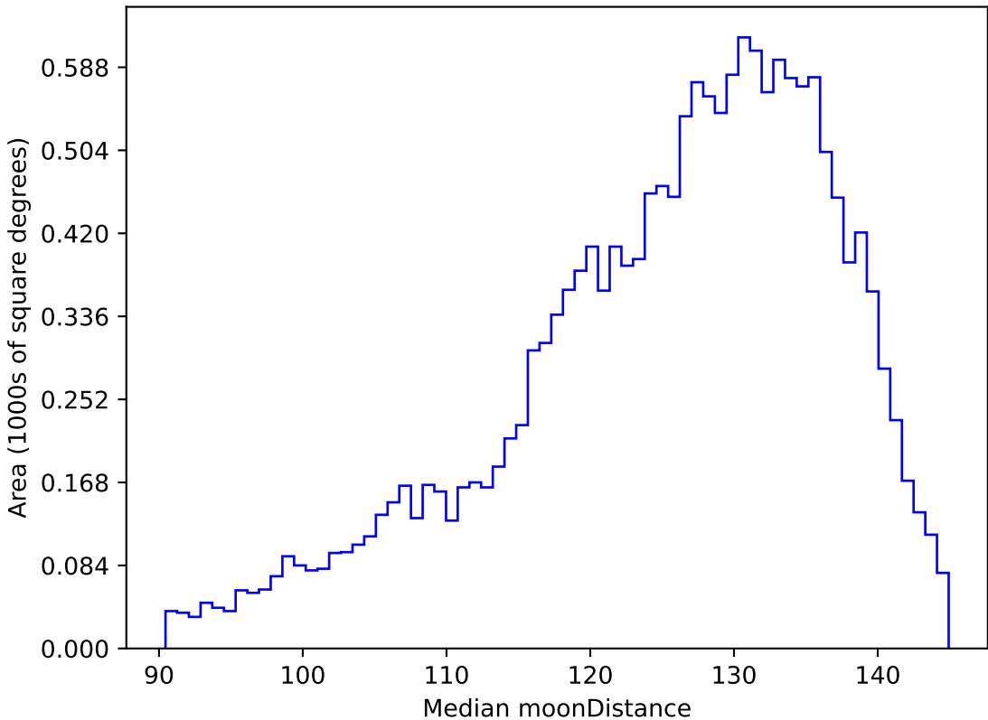
extra_ss_neo4_v3.4_10yrs WFD u band: Median moonDistance
