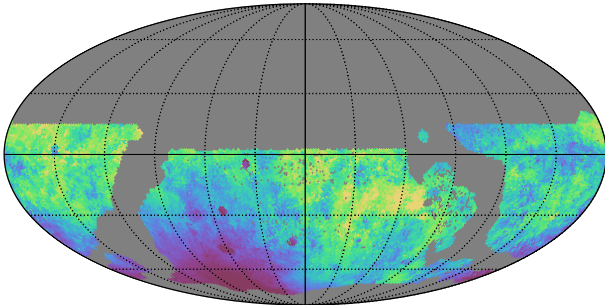
extra_ss_neo4_v3.4_10yrs WFD r band: Median moonDistance
