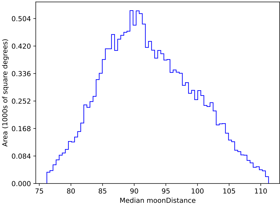
extra_ss_neo4_v3.4_10yrs WFD i band: Median moonDistance
