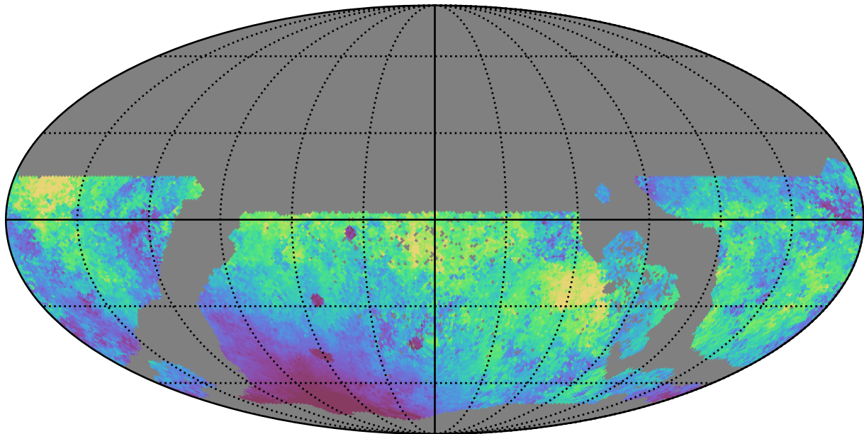
extra_ss_neo4_v3.4_10yrs WFD g band: Median moonDistance
