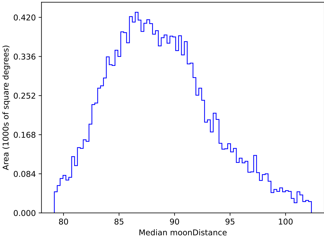
extra_ss_neo4_v3.4_10yrs WFD all bands: Median moonDistance
