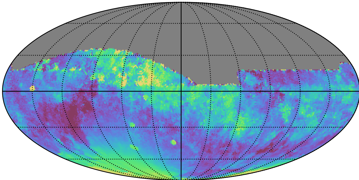
extra_ss_neo4_v3.4_10yrs All sky z band: Median moonDistance
