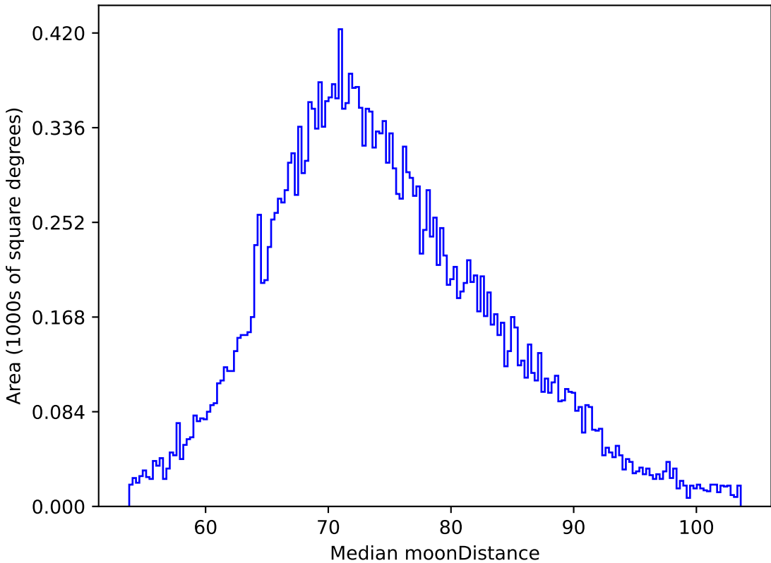
extra_ss_neo4_v3.4_10yrs All sky z band: Median moonDistance
