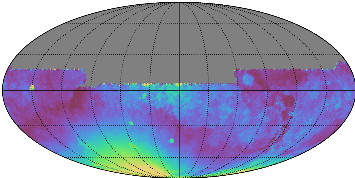
extra_ss_neo4_v3.4_10yrs All sky y band: Median moonDistance
