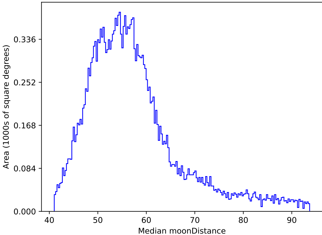
extra_ss_neo4_v3.4_10yrs All sky y band: Median moonDistance
