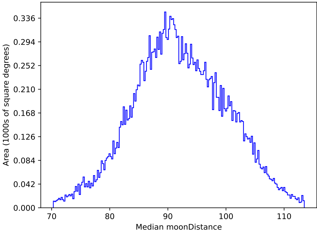
extra_ss_neo4_v3.4_10yrs All sky i band: Median moonDistance
