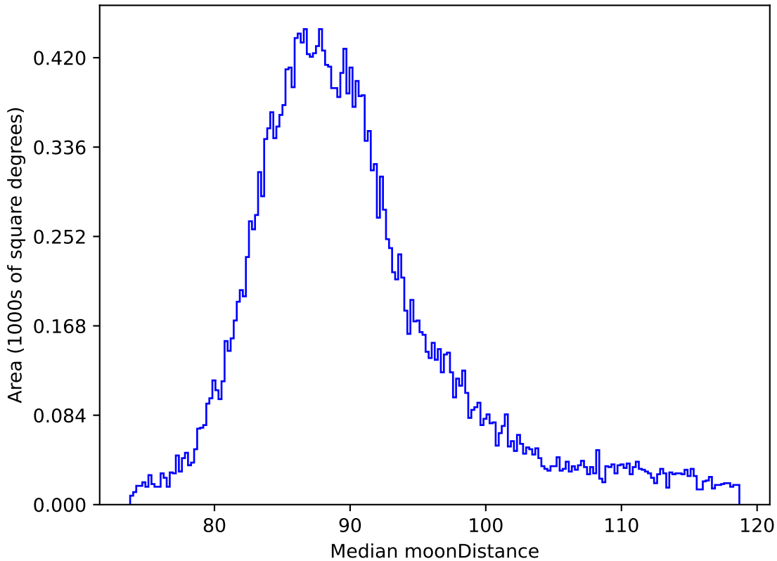
extra_ss_neo4_v3.4_10yrs All sky all bands: Median moonDistance
