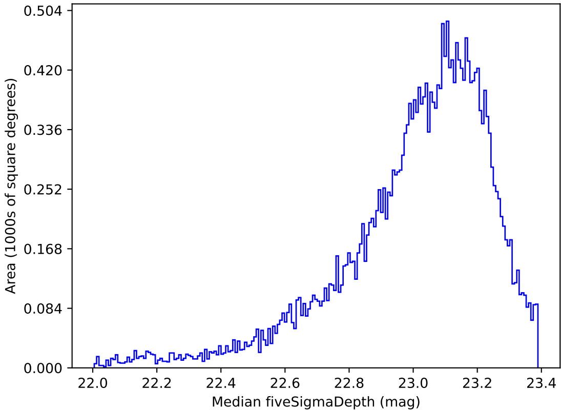
extra_ss_neo4_v3.4_10yrs Yr 1 z band: Median fiveSigmaDepth
