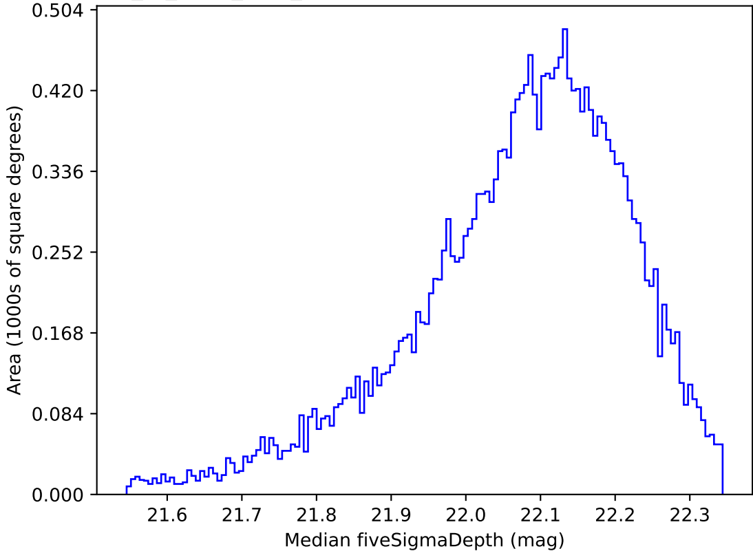
extra_ss_neo4_v3.4_10yrs Yr 1 y band: Median fiveSigmaDepth
