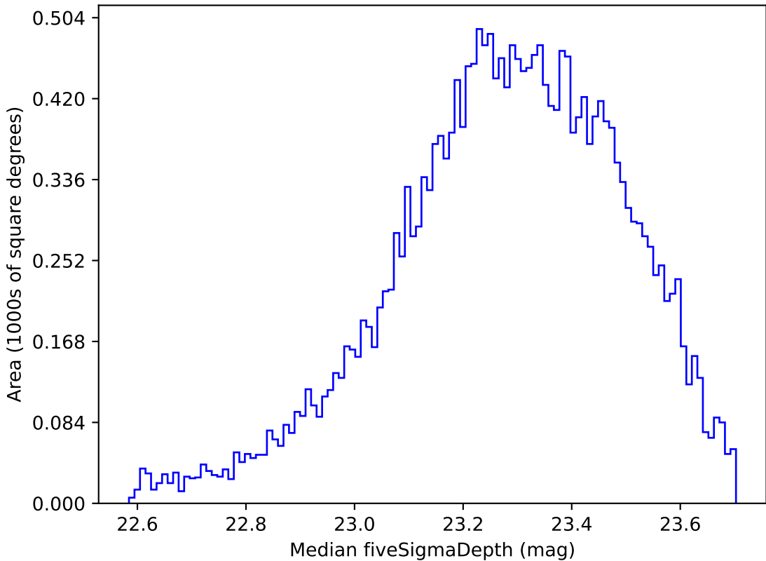
extra_ss_neo4_v3.4_10yrs Yr 1 u band: Median fiveSigmaDepth
