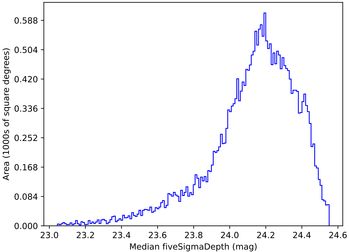
extra_ss_neo4_v3.4_10yrs Yr 1 r band: Median fiveSigmaDepth
