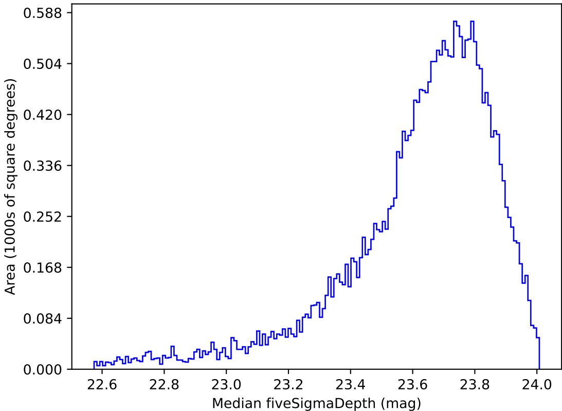
extra_ss_neo4_v3.4_10yrs Yr 1 i band: Median fiveSigmaDepth
