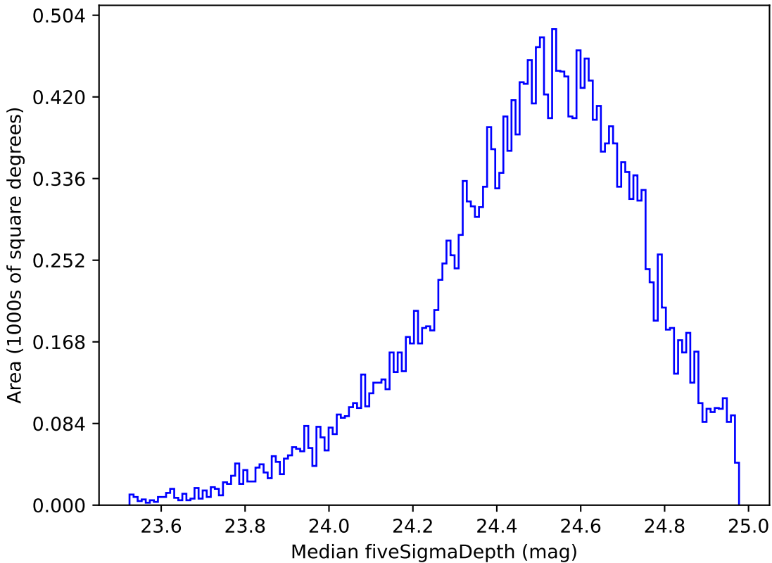
extra_ss_neo4_v3.4_10yrs Yr 1 g band: Median fiveSigmaDepth
