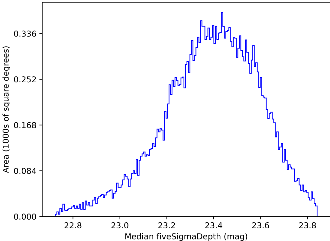
extra_ss_neo4_v3.4_10yrs Yr 1 all bands: Median fiveSigmaDepth
