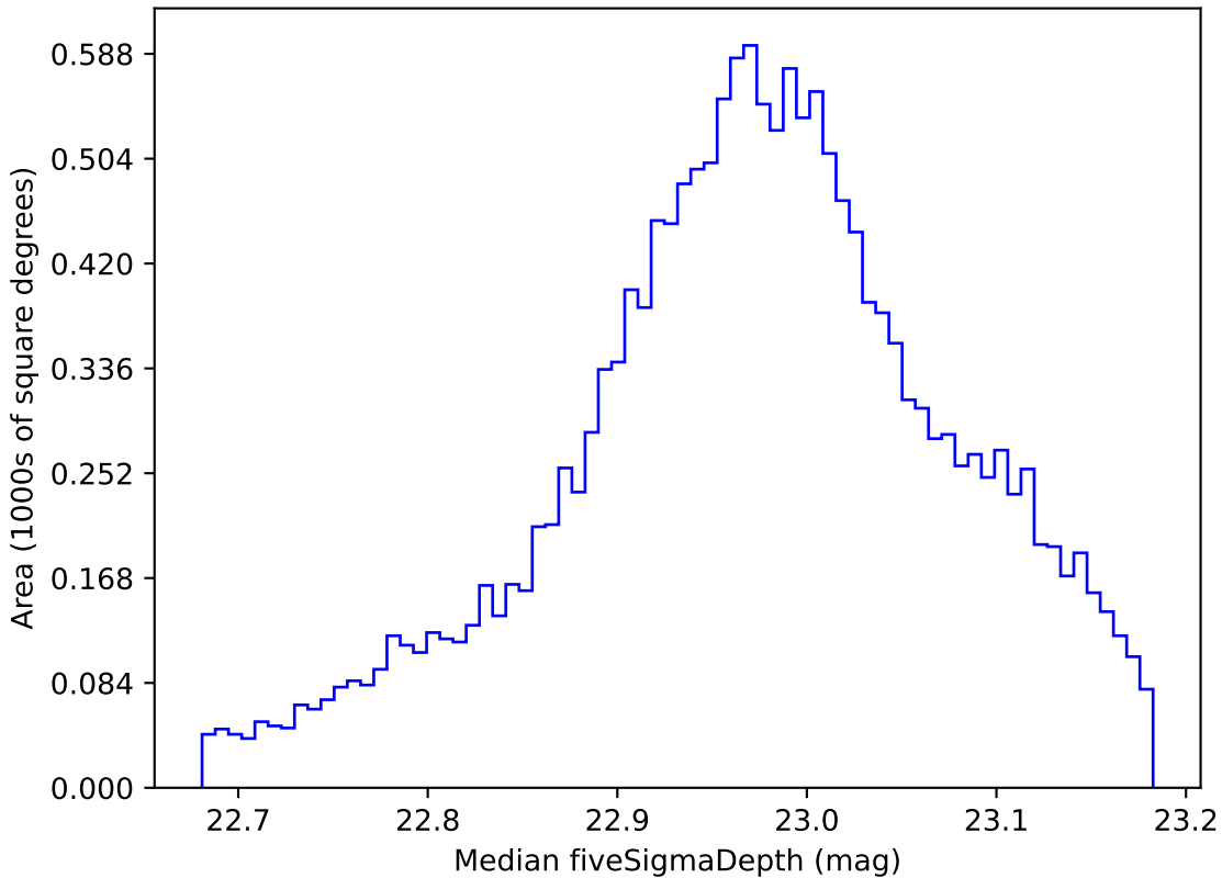
extra_ss_neo4_v3.4_10yrs WFD z band: Median fiveSigmaDepth
