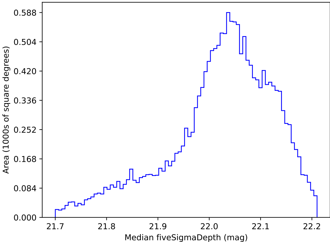
extra_ss_neo4_v3.4_10yrs WFD y band: Median fiveSigmaDepth
