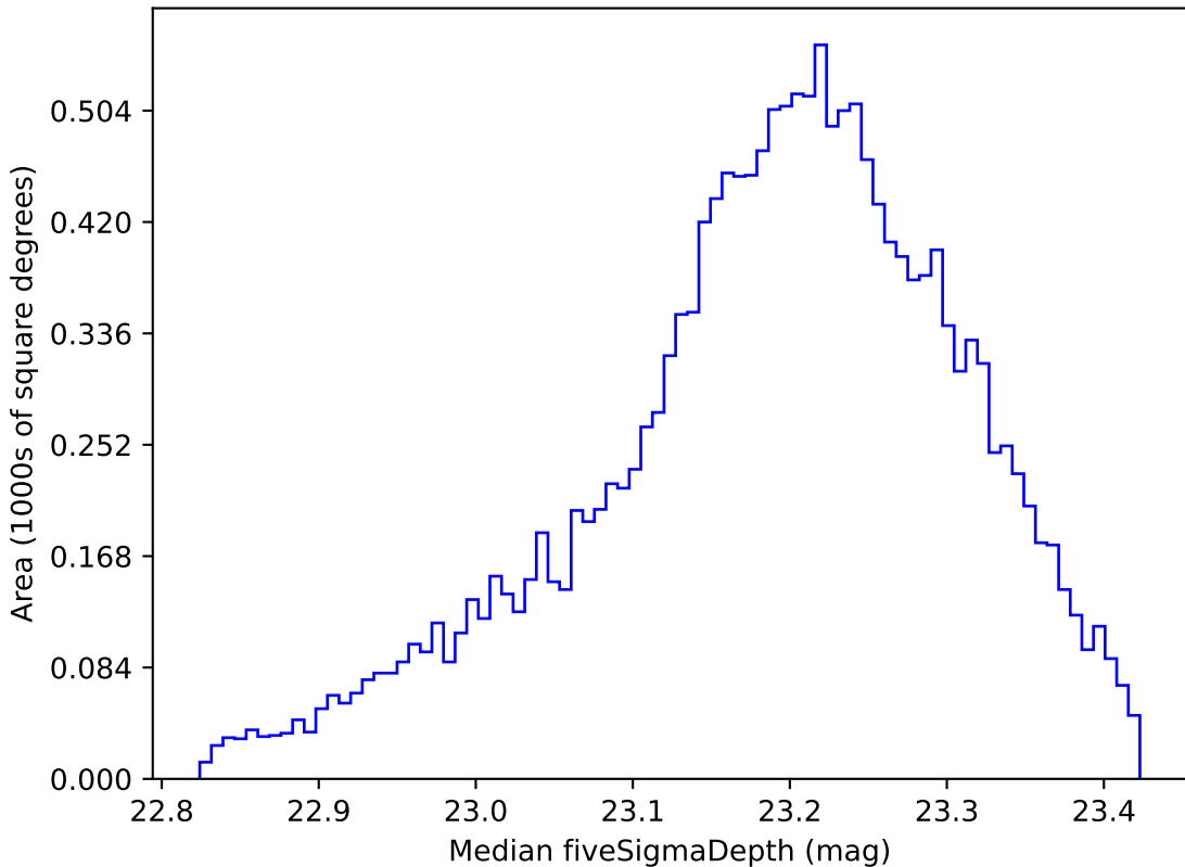
extra_ss_neo4_v3.4_10yrs WFD u band: Median fiveSigmaDepth
