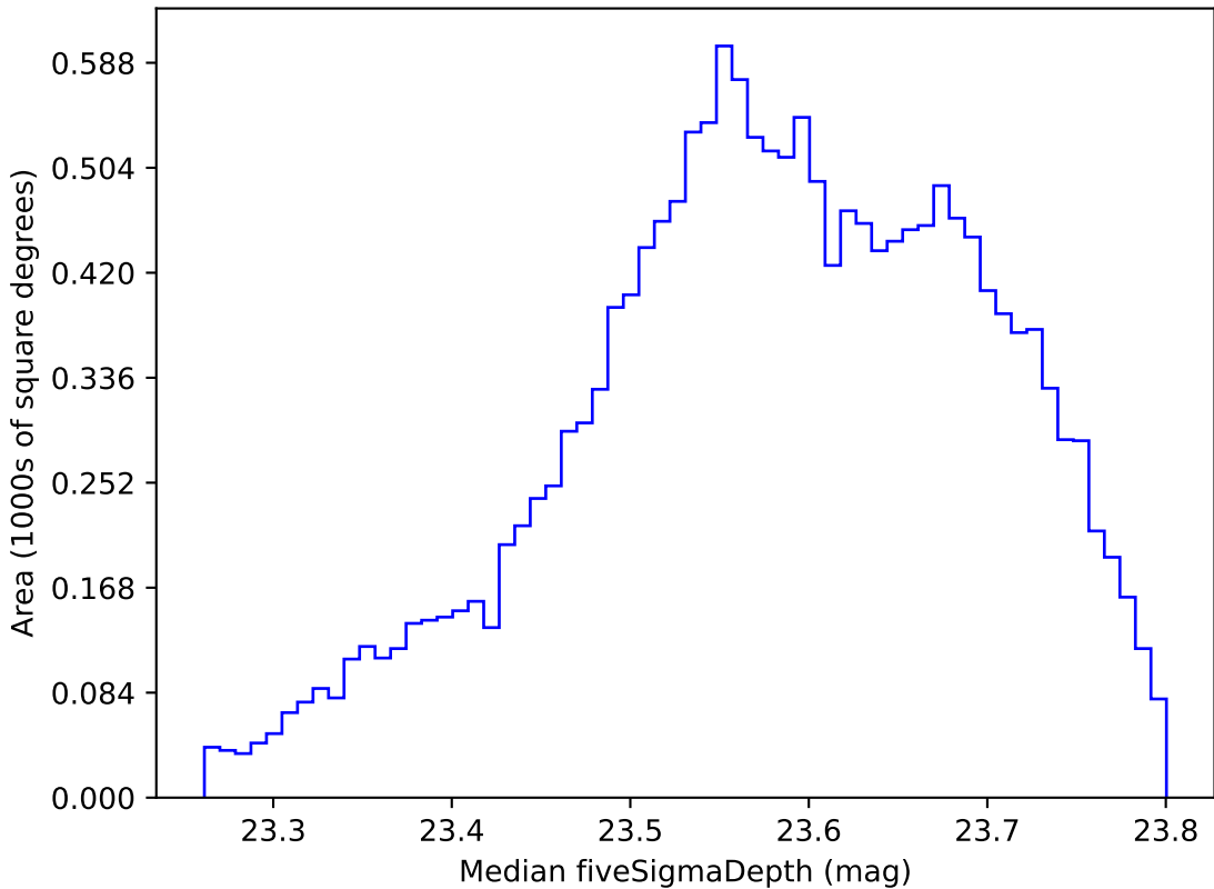
extra_ss_neo4_v3.4_10yrs WFD i band: Median fiveSigmaDepth
