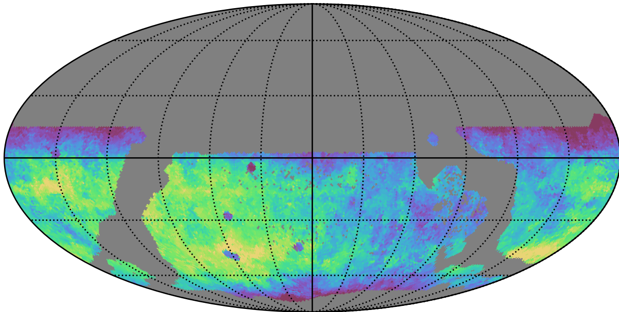
extra_ss_neo4_v3.4_10yrs WFD g band: Median fiveSigmaDepth
