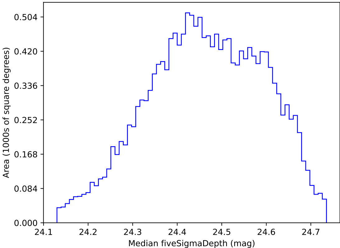
extra_ss_neo4_v3.4_10yrs WFD g band: Median fiveSigmaDepth
