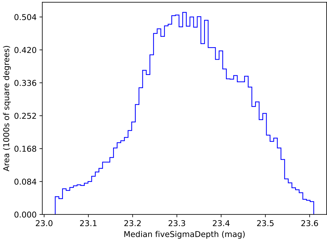
extra_ss_neo4_v3.4_10yrs WFD all bands: Median fiveSigmaDepth
