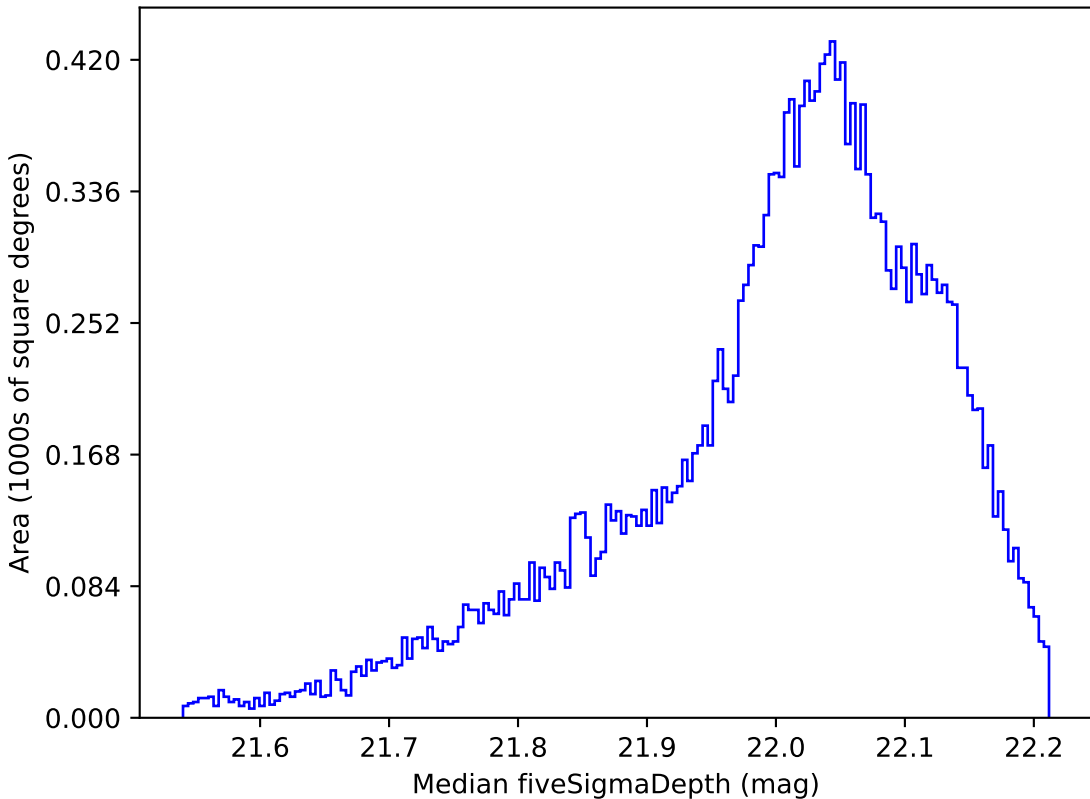
extra_ss_neo4_v3.4_10yrs All sky y band: Median fiveSigmaDepth
