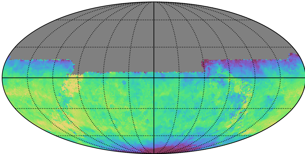
extra_ss_neo4_v3.4_10yrs All sky u band: Median fiveSigmaDepth
