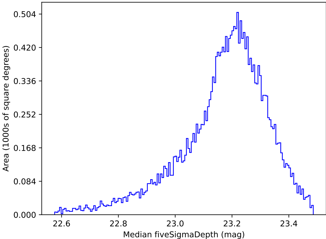
extra_ss_neo4_v3.4_10yrs All sky u band: Median fiveSigmaDepth
