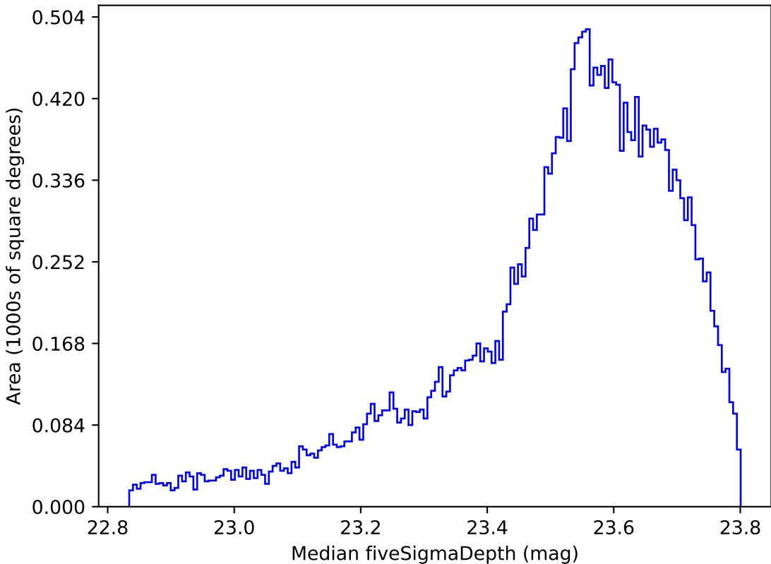
extra_ss_neo4_v3.4_10yrs All sky i band: Median fiveSigmaDepth
