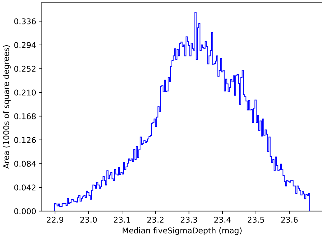
extra_ss_neo4_v3.4_10yrs All sky all bands: Median fiveSigmaDepth
