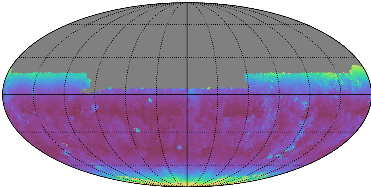
extra_ss_neo4_v3.4_10yrs Yr 1 y band: Median airmass
