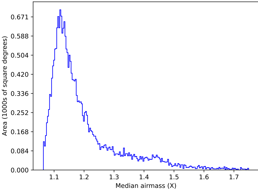
extra_ss_neo4_v3.4_10yrs Yr 1 y band: Median airmass
