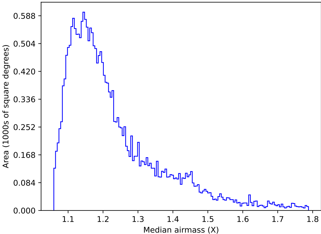
extra_ss_neo4_v3.4_10yrs Yr 1 u band: Median airmass
