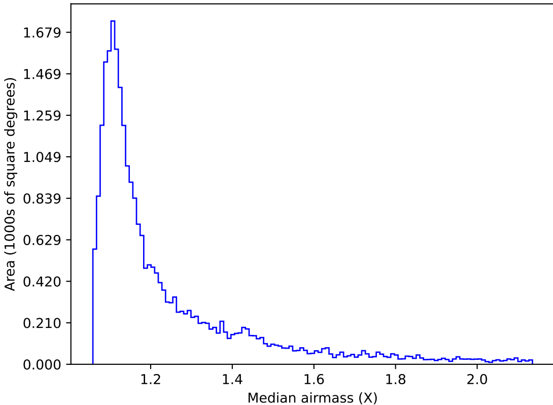
extra_ss_neo4_v3.4_10yrs Yr 1 r band: Median airmass
