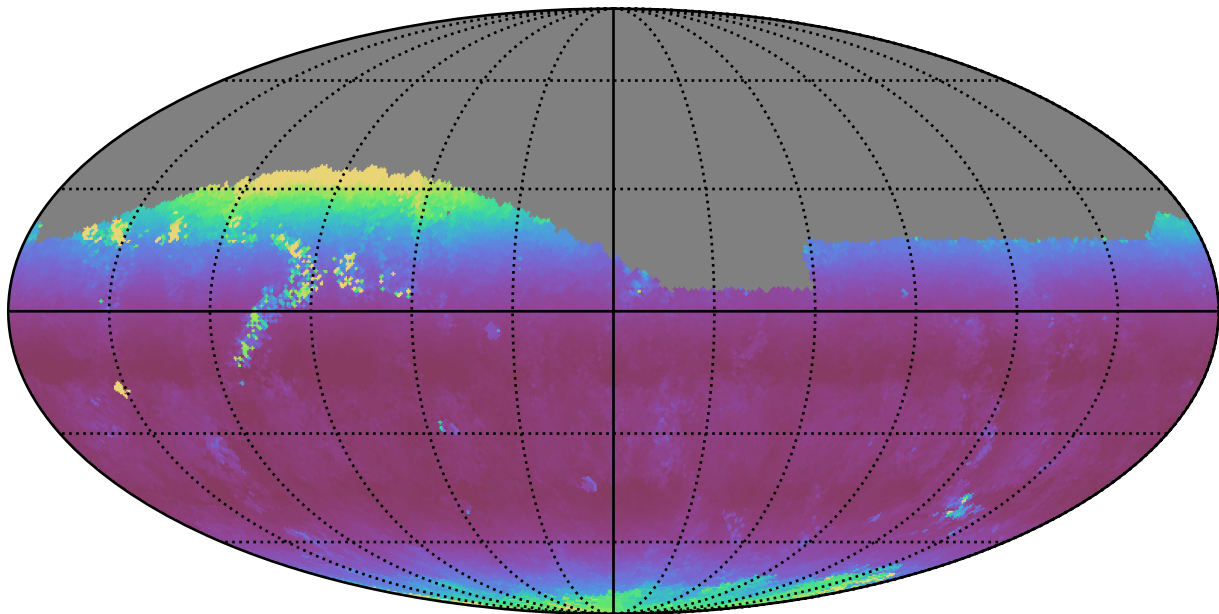
extra_ss_neo4_v3.4_10yrs Yr 1 i band: Median airmass
