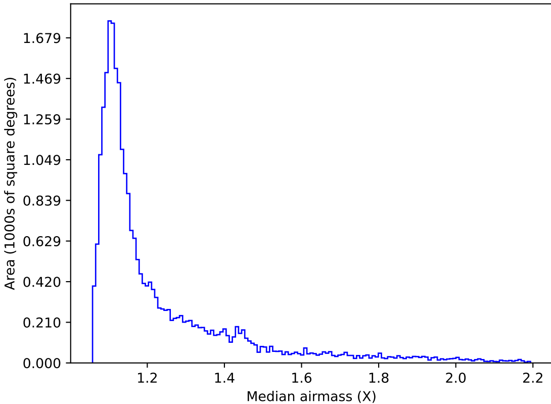
extra_ss_neo4_v3.4_10yrs Yr 1 i band: Median airmass
