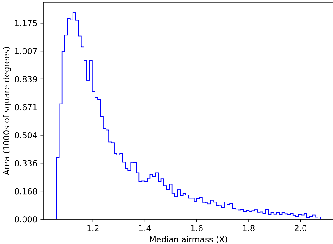
extra_ss_neo4_v3.4_10yrs Yr 1 g band: Median airmass
